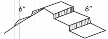
RIDGE CAP
