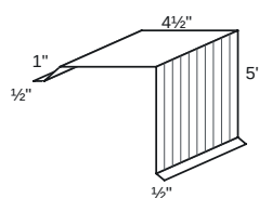
Gable end trim
