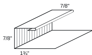
J-channel
