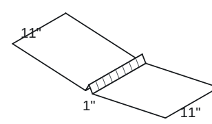
W-valley
