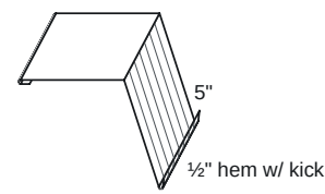
Swept wing gable end
