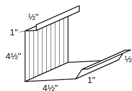
Outside corner cap
