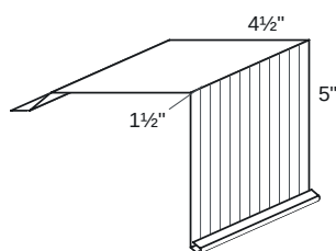
Gable end
