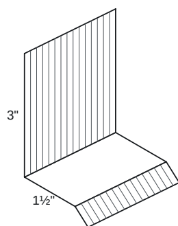
Rat guard
