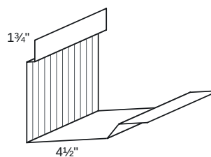
Outside corner
